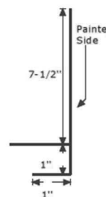
Overhead Door Trim
